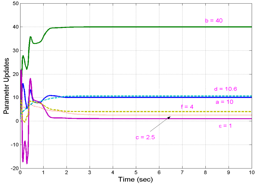
Figure 3. Parameter Estimates \hat{a}(t) , \hat{b}(t) , \hat{c}(t) , \hat{d}(t) , \hat{\epsilon}(t) , \hat{f}(t)
