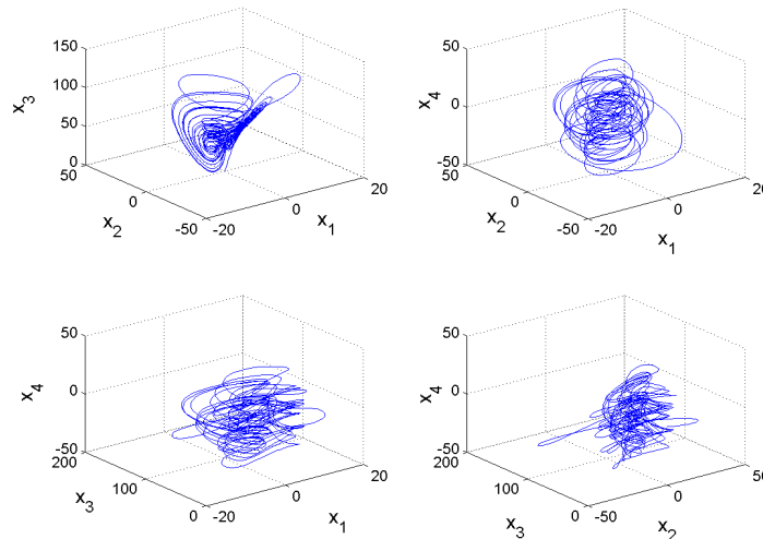
Figure 1. State Orbits of the Hyperchaotic Liu System
