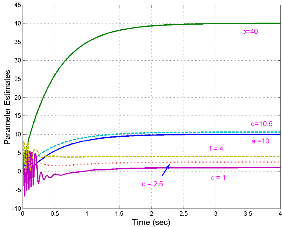
Figure 5. Parameter Estimates \hat{a}(t) , \hat{b}(t) , \hat{c}(t) , \hat{d}(t) , \hat{\epsilon}(t) , \hat{f}(t)
