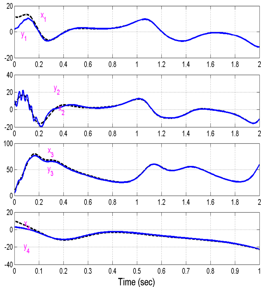
Figure 4. Adaptive Synchronization of the Identical Hyperchaotic Liu Systems
