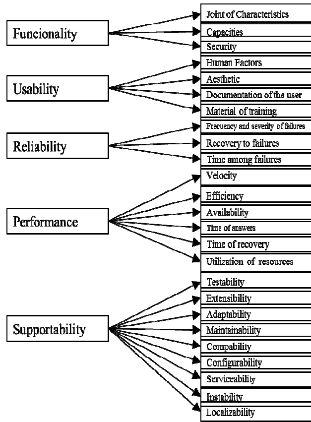
Figure 5 FURPS Model
