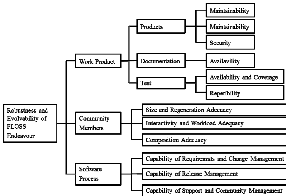
Figure 18 – QualOSS Model
