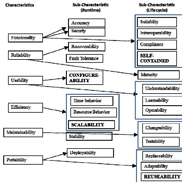
Figure 13. Alvaro Model
