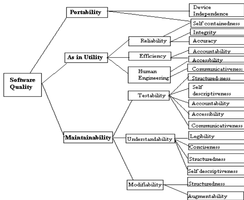
Figure 3 – Boehm Model -1978
