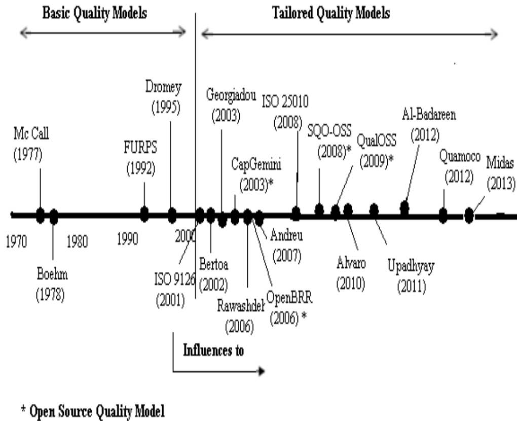
Figure 1 Quality Models
