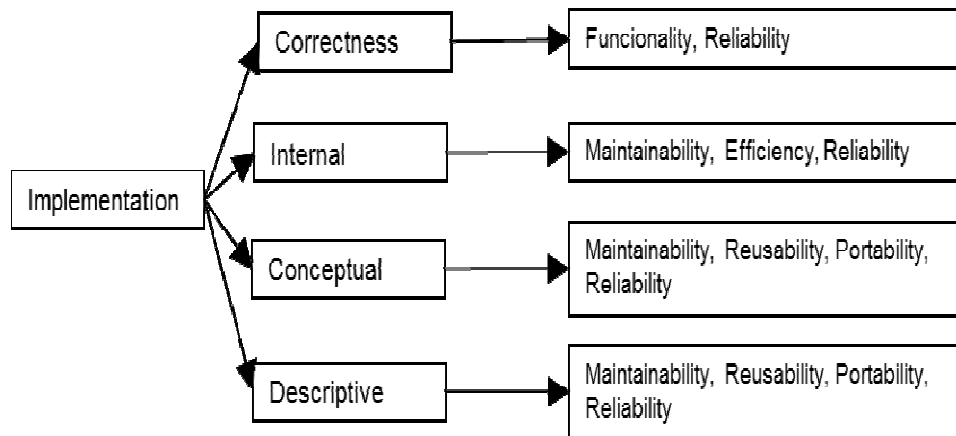
Figure 4 Dromey Model
