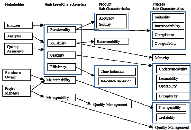
Figure 14– Rawashdeh Model
