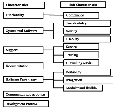
Figure 16 OpenBRR model
