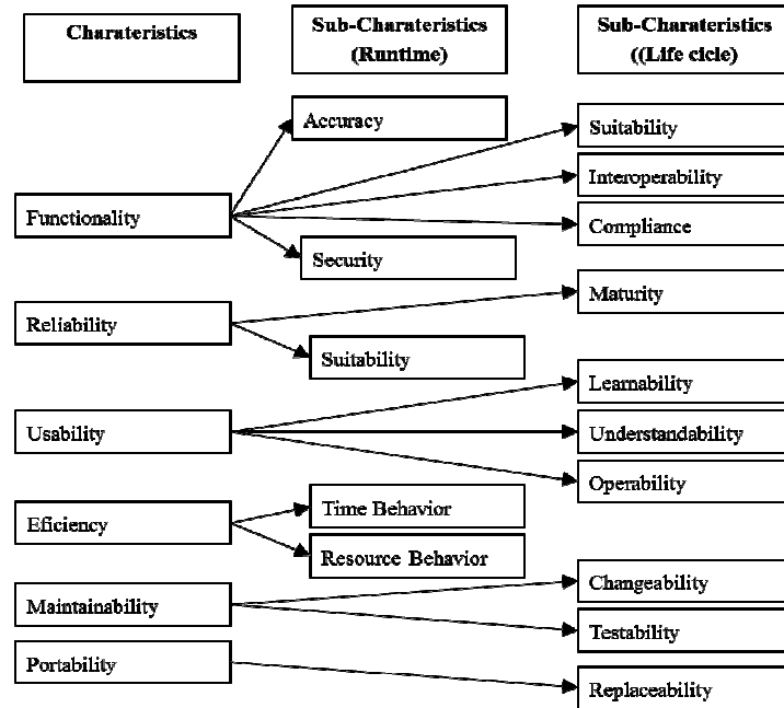
Figure 11 Bertoa Model
