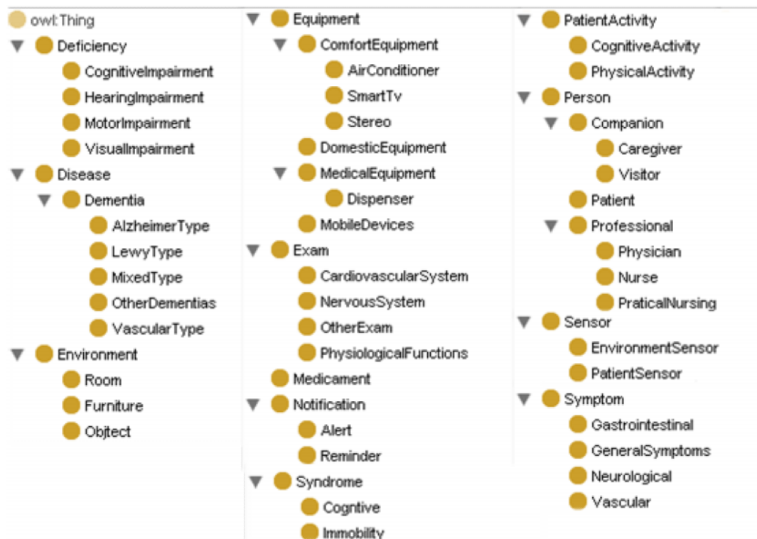
Figure 1. Classes of the proposed ontology
