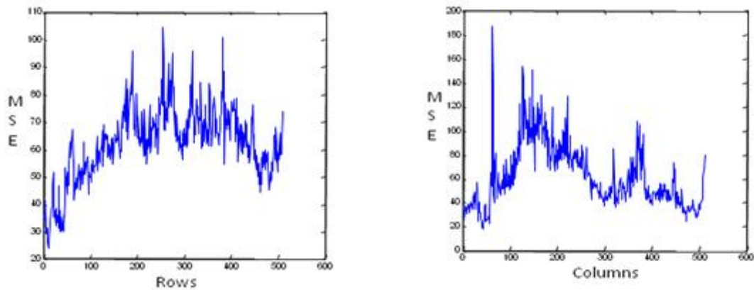
Figure 2. Average MSE for each row and column of the 512 \times 512 Lena image after compression at a bit rate of 0.1 bits-per-pixel using JPEG2000 Part1 with tile size of 64 \times 64 .
