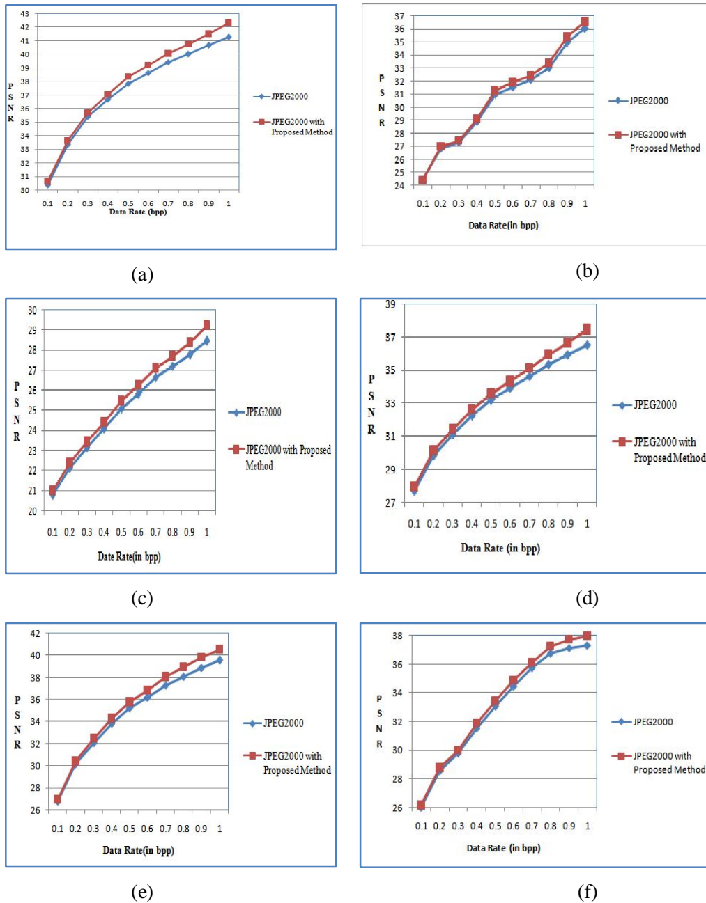
Figure 4. PSNR comparison of (a) Lena (b) Barbara (c) Baboon (d) Gold Hill (e) Airplane and (f) Bike images compressed at different bit rates using JPEG2000 standard and JPEG2000 standard with proposed post-processing method.
