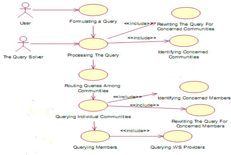
Figure 2. UML Use Case diagram for querying communities
