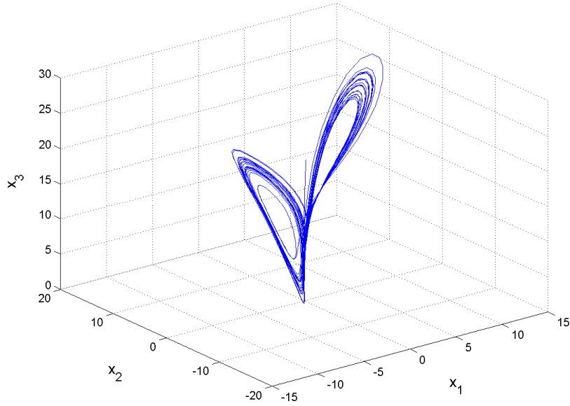
Figure 1. Strange Attractor of the Pan System
