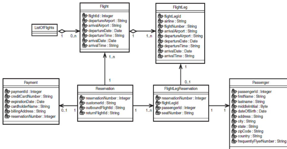
Figure 1.8 Class Reservation and related classes
