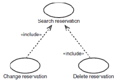
Figure 1.3 an include relationship between two use cases
