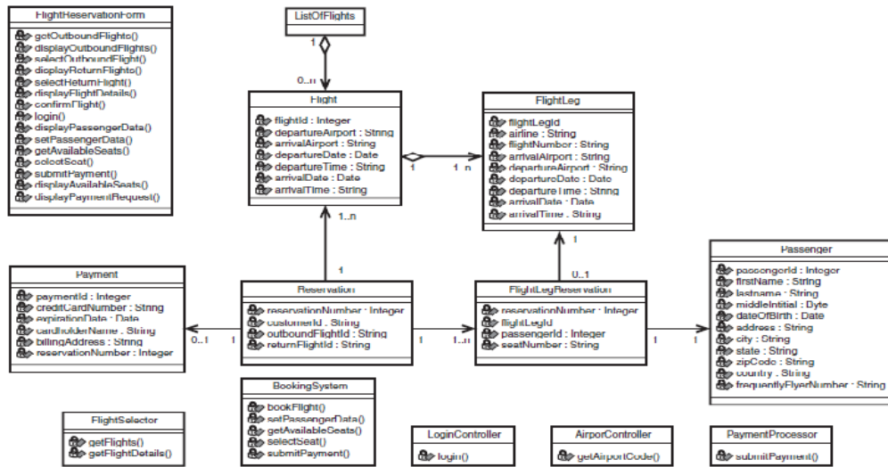
Figure 1.7 A class diagram showing classes that implement the functionality of a basic flow of the Book a flight use case.
