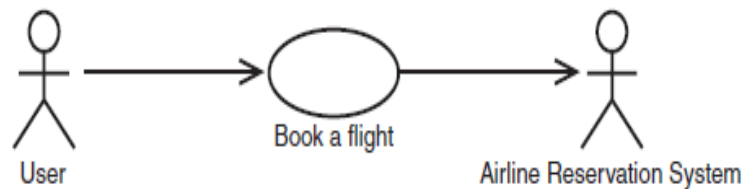
Figure 1.5 A Context diagram for the Use case book a flight
