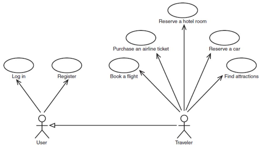
Figure 1.2 Use case Initiated by Travellers and User
